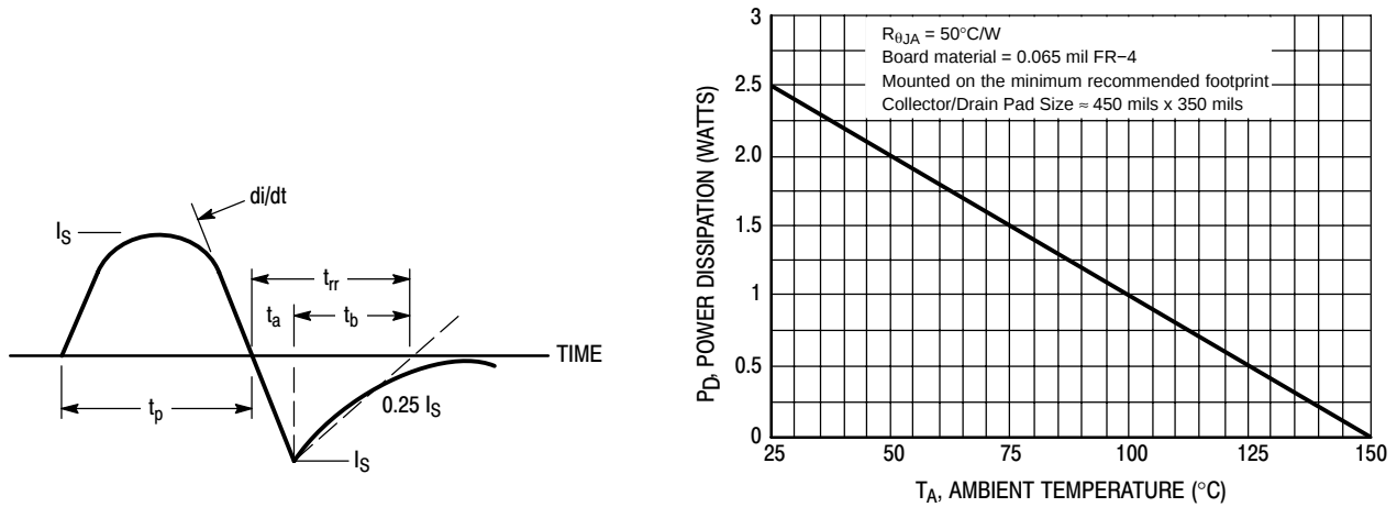
Figure 15. Diode Reverse Recovery Waveform
